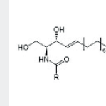
Ceramide NP
